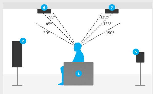
Overhead speaker placement detail for 5.1.4 setup
