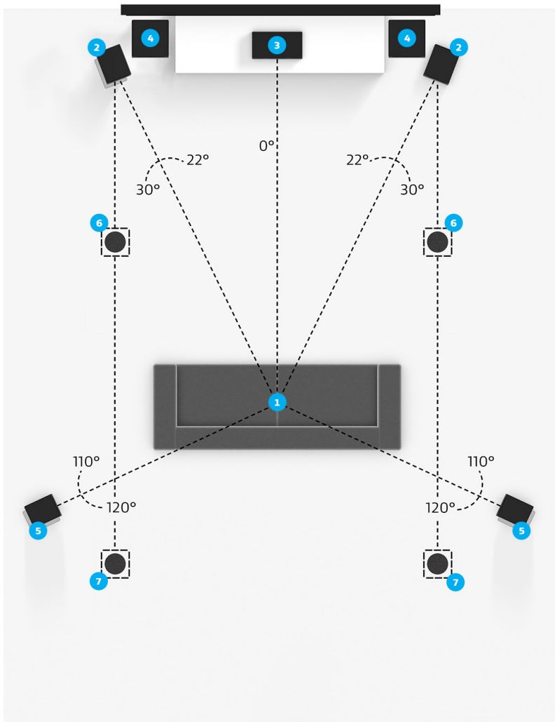
Speaker placement for 5.1.4 setup
